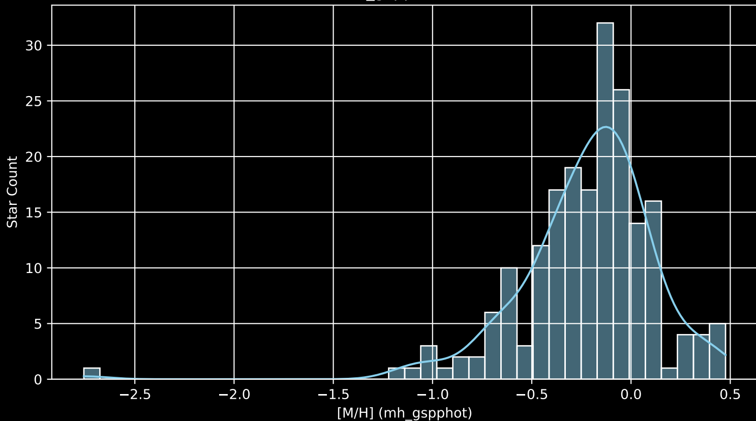
APOGEE DR17 Field: [087-41_MGA [M/H] (mh_gspphot) (n= 197)
