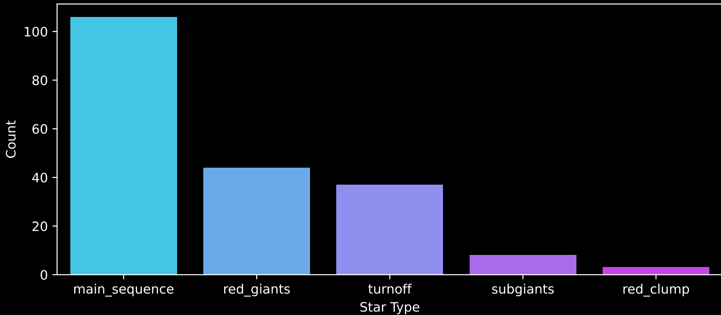
APOGEE DR17 Field: [087-41_MGA] Count plot of Star Type
