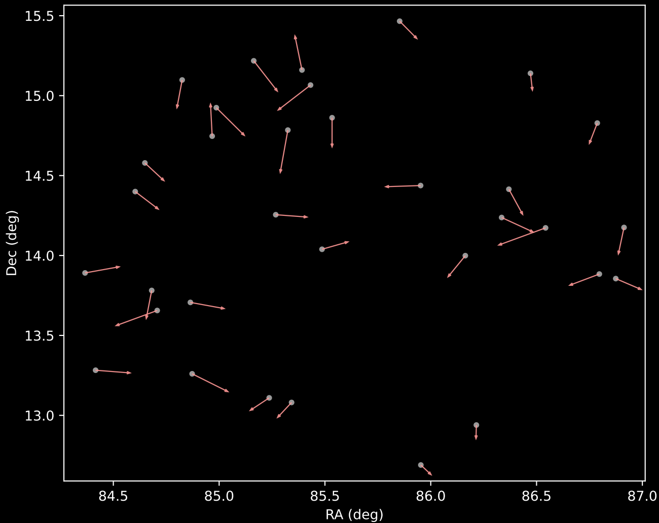
APOGEE DR17 Cluster 7 Proper Motion Vectors (n=33)
