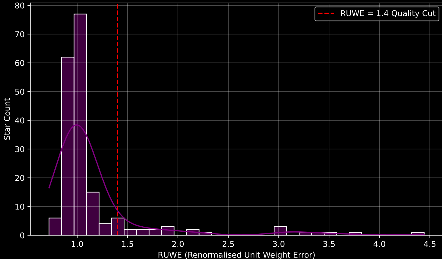
GAPOGEE DR17 Field [087-41_MGA] RUWE Distribution (n= 190)
