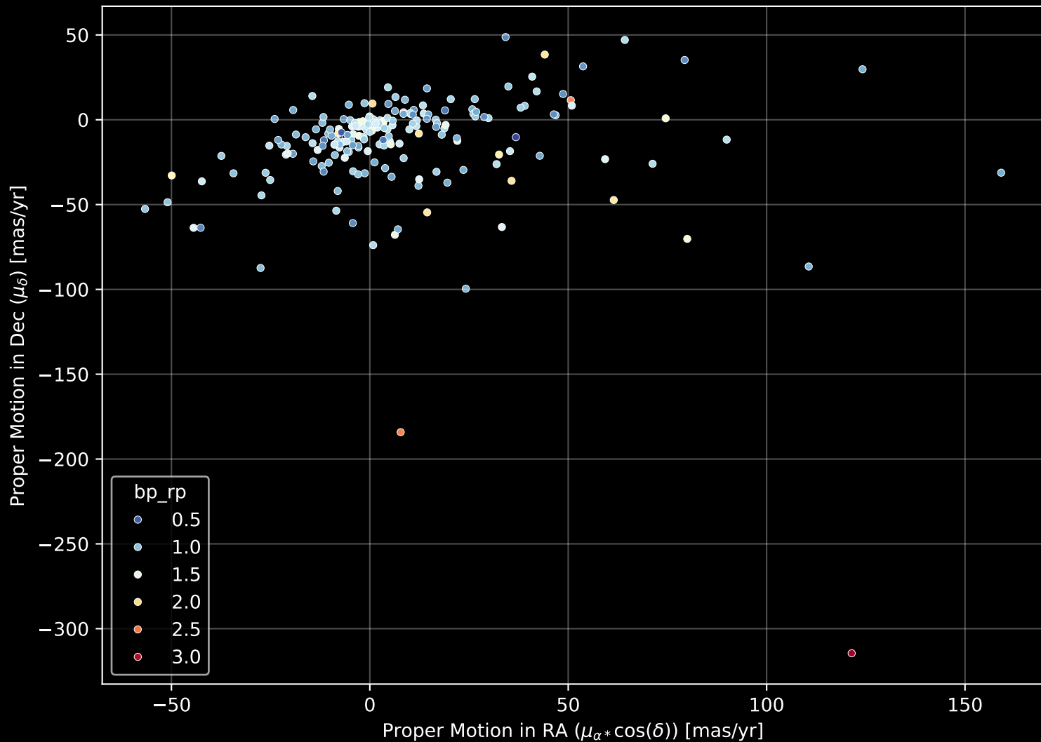
APOGEE DR17 Field: [087-41_MGA] Proper Motion Diagram (n= 198)
