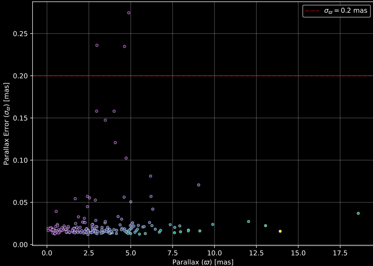
APOGEE DR17 Field: [087-41_MGA] Parallax Quality (n= 198)
